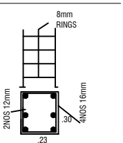
COLUMN DETAILS
