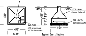
FOOTING DETAILS
