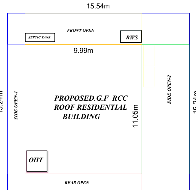
15.54m SITE PLAN
