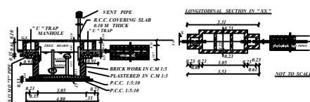
SEPTICK TANK & DISPERSION TRINCH
