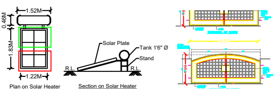
Plan on Solar Heater
