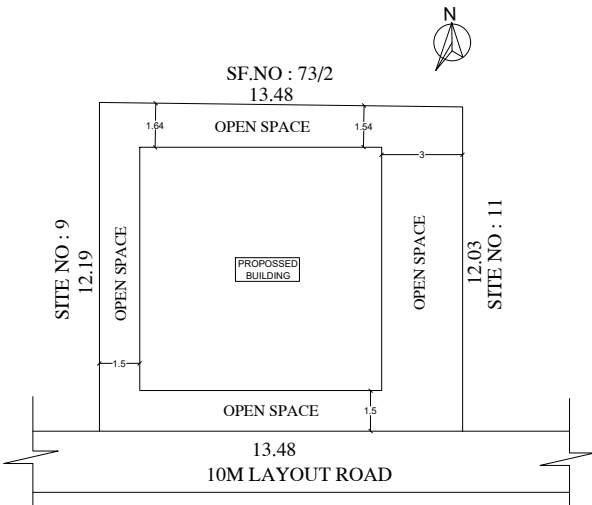
SITE PLAN
