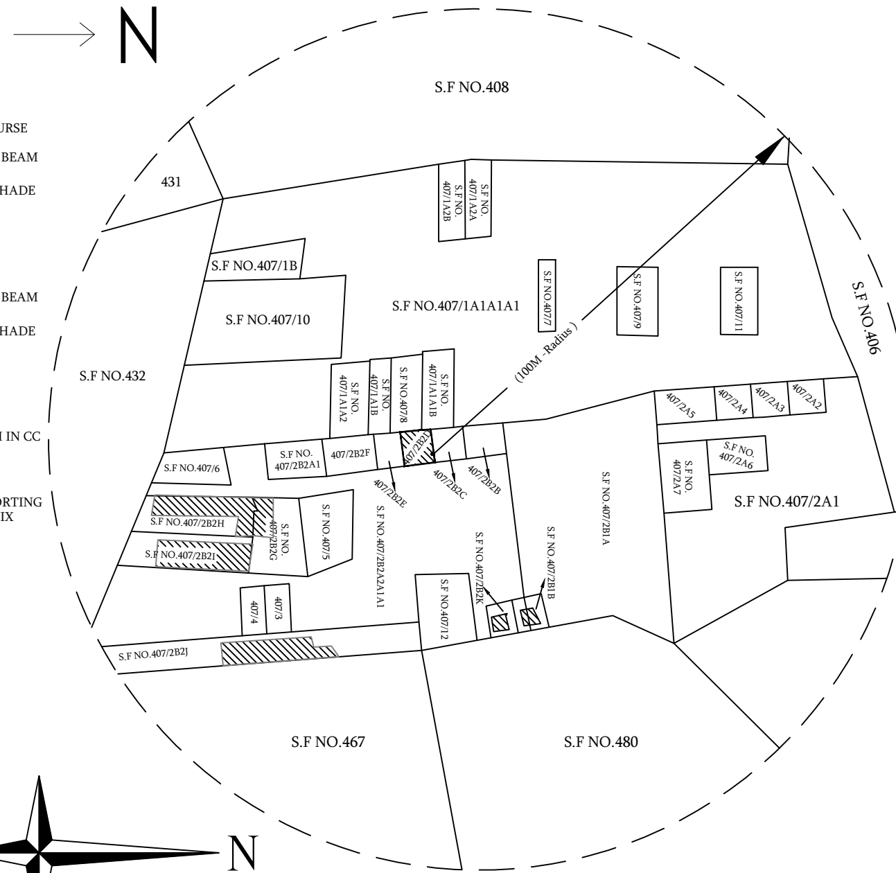
TOPO SKETCH (OR) KEY PLAN
