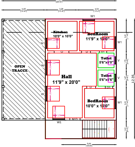
RCC ROOF RESIDENTIAL BUILDING IN PROPOSED FIRST FLOOR PLAN
