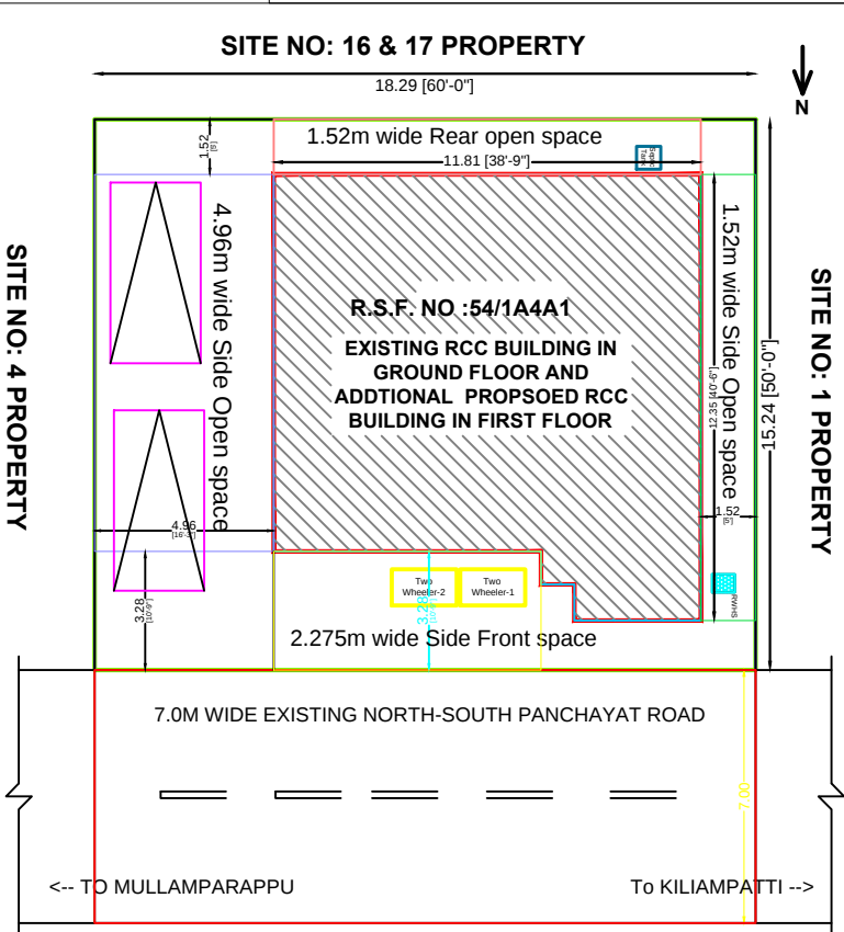
SITE PLAN (1:100)
