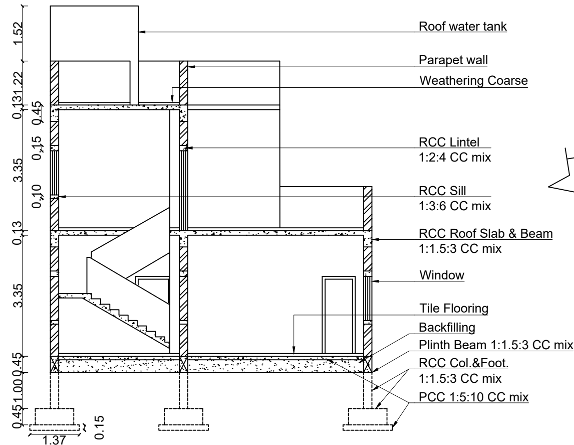
SECTION "AA"
