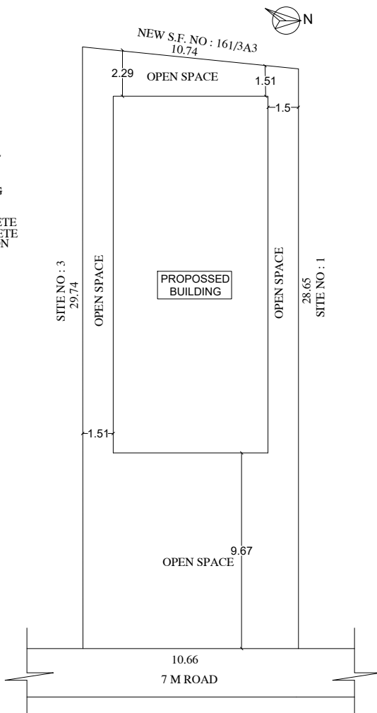
SITE PLAN
