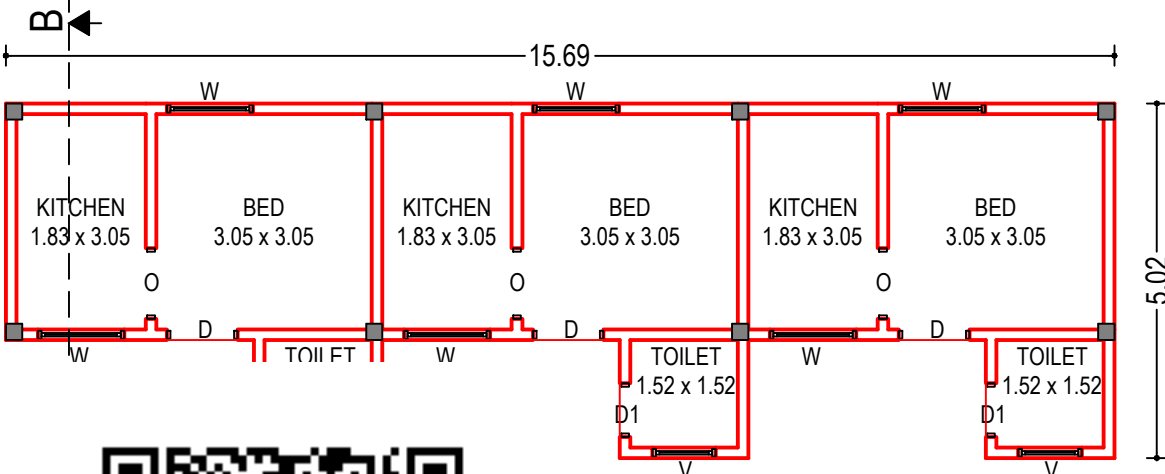
FLOOR PLAN
