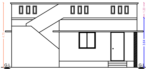
EXISTING PRO. BUILDING FRONT ELEVATION
