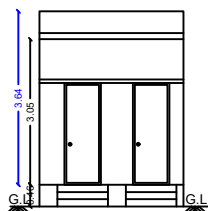
ADDITIONAL PRO. FRONT ELEVATION
