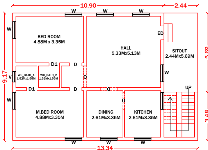
EXISTING PRO. BUILDING GROUND FLOOR PLAN
