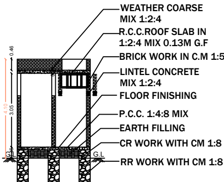
ADDITIONAL PRO. SECTION - AB
