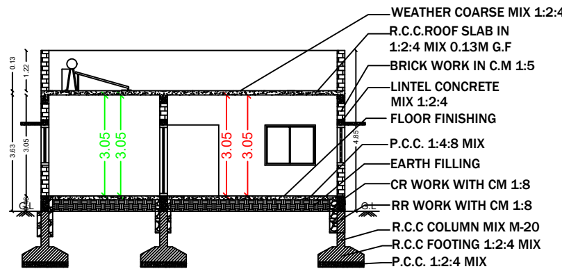
EXISTING PRO. BUILDING SECTION - AA
