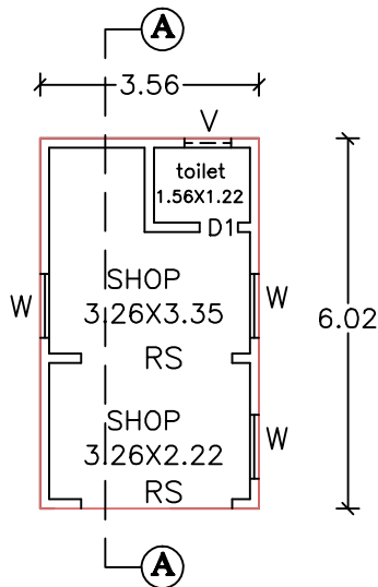
PLAN (SCALE 1:100)
