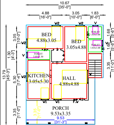
GROUND FLOOR PLAN (EAST)
