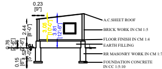
SECTION ON "AA"
