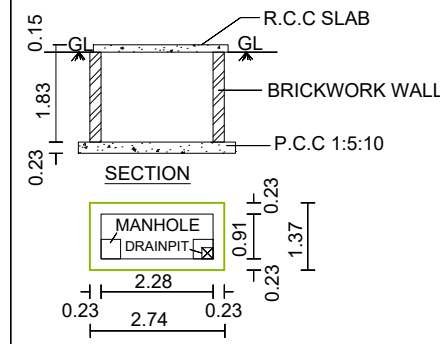
SUMP DETAILS
