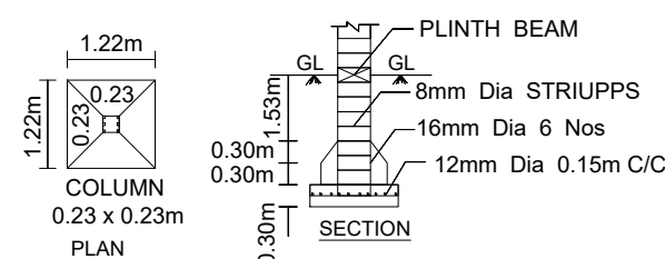
COLUMN FOUNDATION DETAILS
