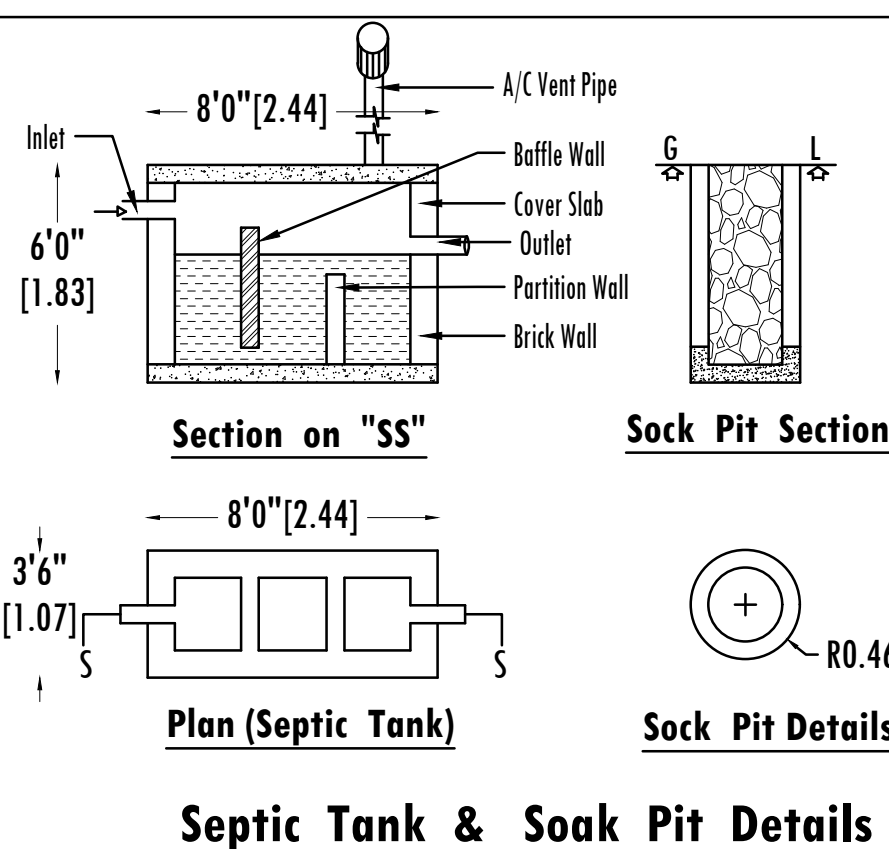
Septic Tank & Soak Pit Details
