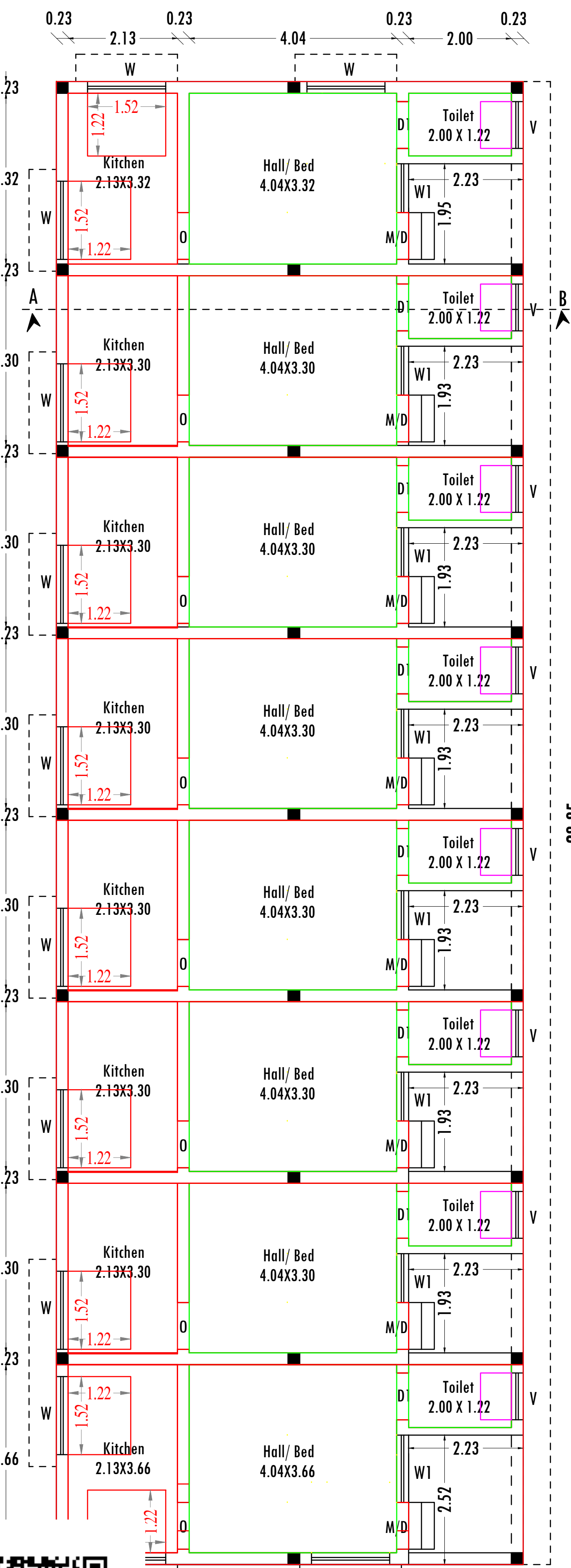
Ground Floor Scale:- 1:100
