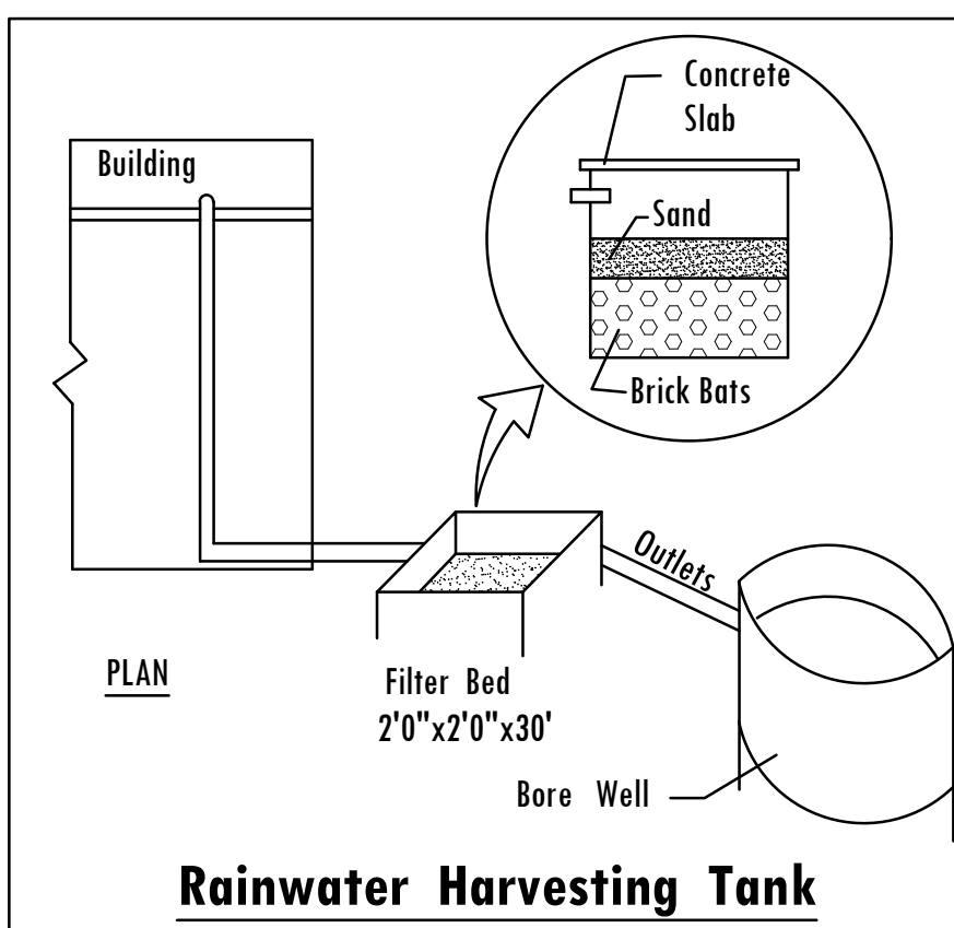
Rainwater Harvesting Tank
