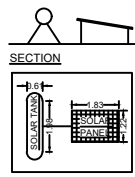
SOLAR SYSTEM
