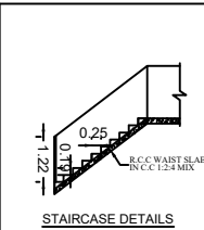
STAIRCASE DETAILS
