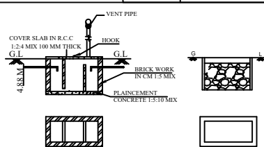
SEPTIC TANK DETAILS
