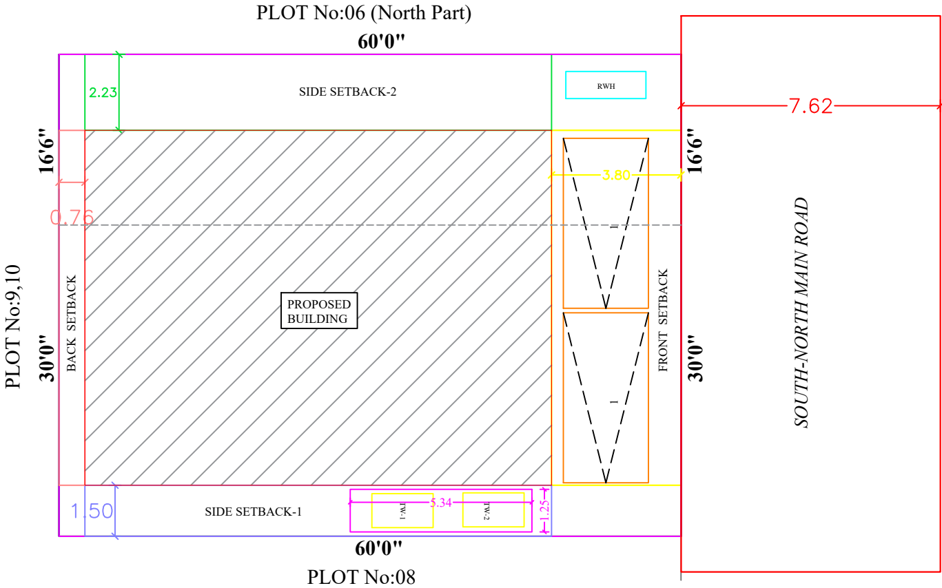
SITE PLAN
