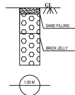
DETAILS OF RAINWATER HARVESTING TANK. (NTS)
