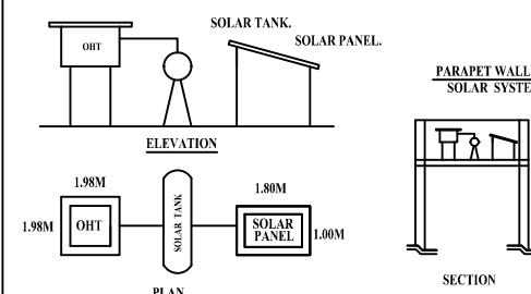
DETAILS OF SOLAR ENERGY SYSTEM
