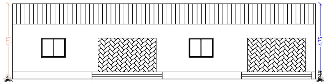
FRONT ELEVATION
