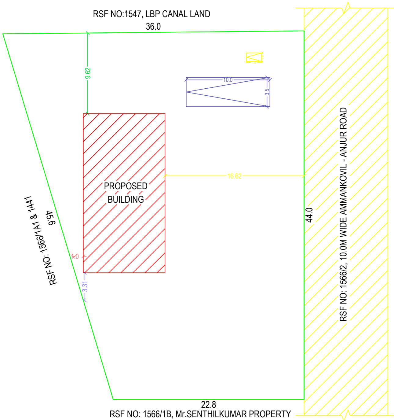
SITE PLAN
