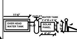
SOLAR WATER HEATER DETAILS
