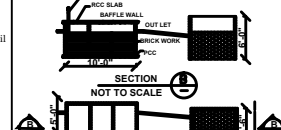
SEPTIC TANK WITH DISPERSION TRENCH
