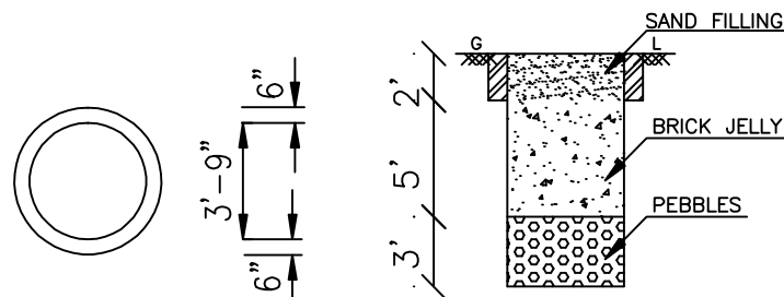
RAIN WATER HARVESTING SYSTEM SCALE 1:50
