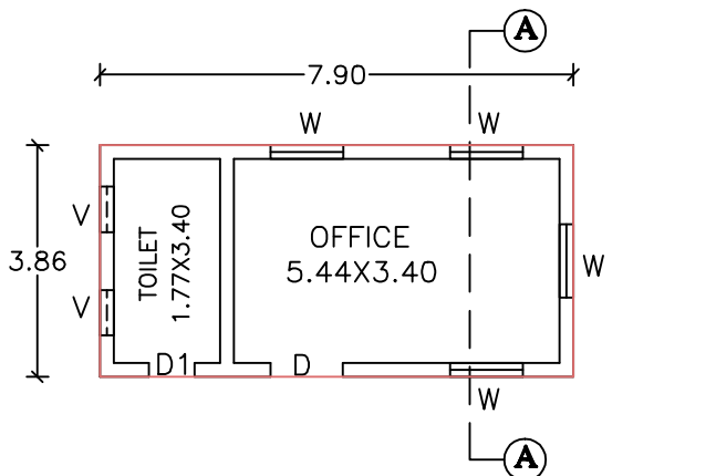
GROUND FLOOR PLAN (SCALE 1:100)
