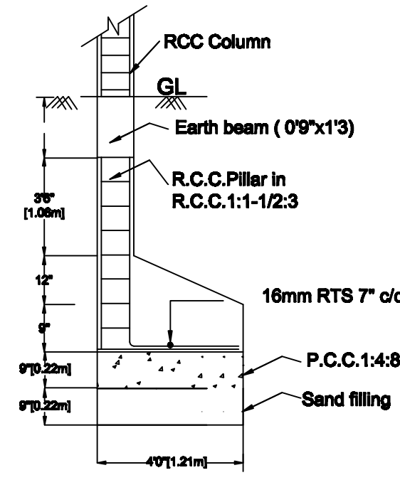
FOUNDATION DETAILS
