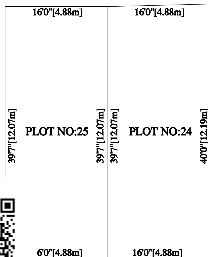
9.00m WIDE ROAD DETAILED SITE PLAN
