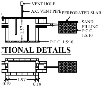
WATER TANK DETAILS
