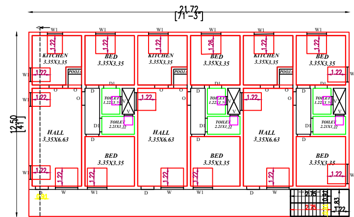
GROUND FLOOR PLAN (SCALE 1:100)
