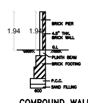
COMPOUND WALL
