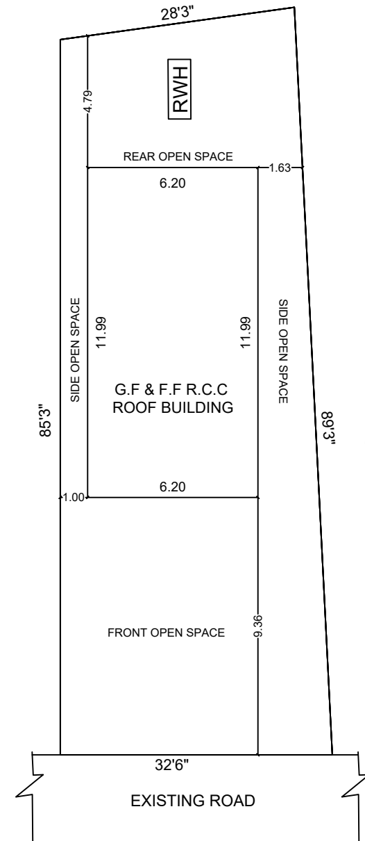
SITE PLAN
