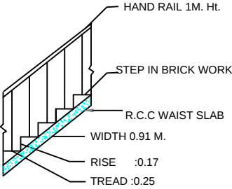
STAIR DETAIL
