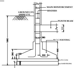
FOUNDATION DETAILS
