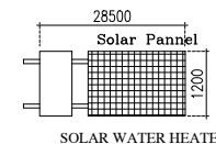
SOLAR WATER HEATER (Not to scale)
