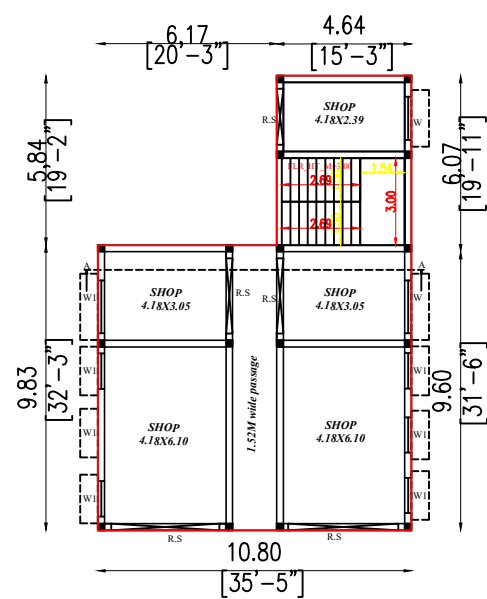
GROUND FLOOR PLAN EXISTING BUILDING
