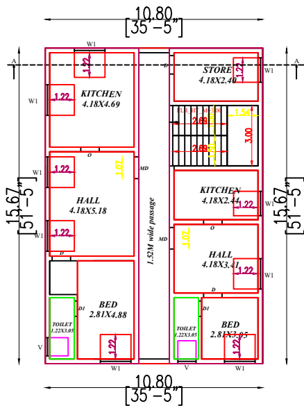
FIRST FLOOR PLAN PROPOSED BUILDING (SCALE 1:100)
