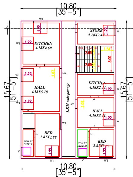
SECOND FLOOR PLAN PROPOSED BUILDING (SCALE 1:100)
