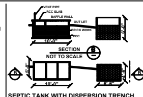
SEPTIC TANK WITH DISPERSION TRENCH
