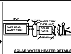
SOLAR WATER HEATER DETAILS
