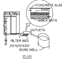
RAIN WATER HARVESTING TANK
