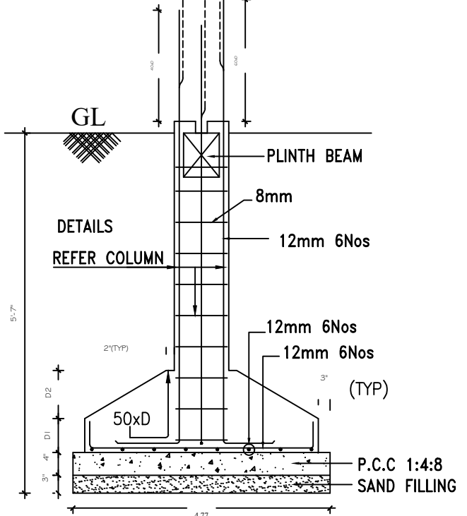
FOUNDATION - COLUMN DETAILS (Not To Scale)
