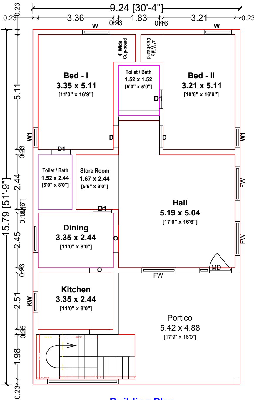
Building Plan Ground Floor
