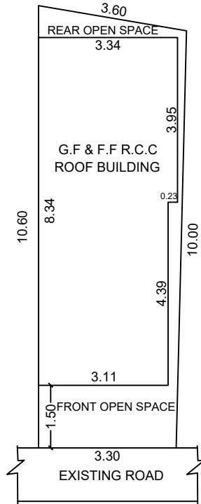
SITE PLAN
