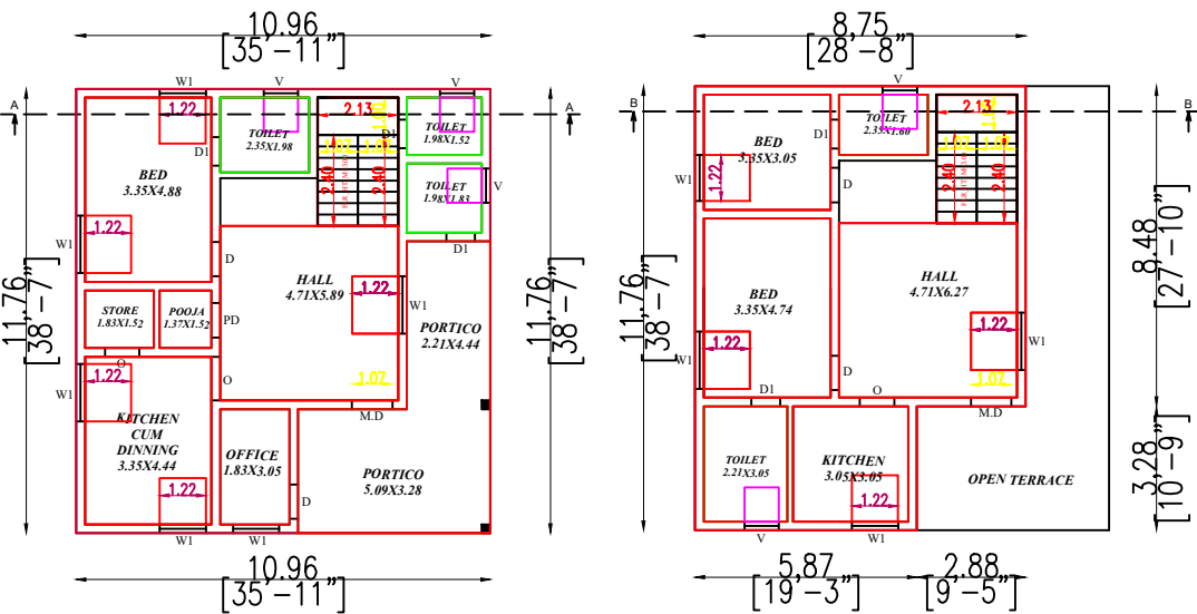
GROUND FLOOR PLAN PROPOSED BUILDING (SCALE 1:100)
