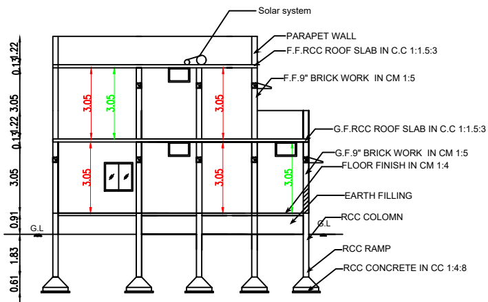
SECTION ON AA&BB
