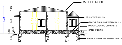
SECTION A - B
