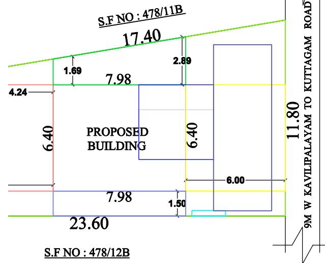
SITE PLAN
