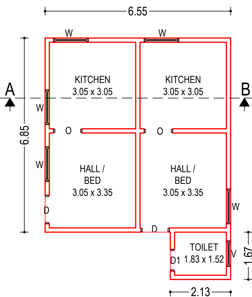
PLAN
