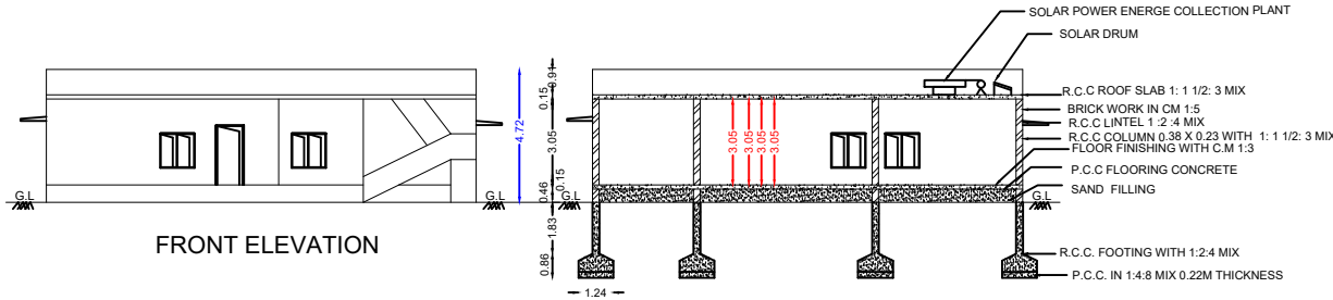
SECTION A - B
