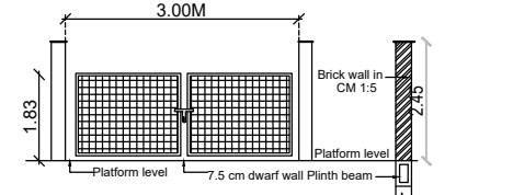
Gate Elevation & Cross Section
