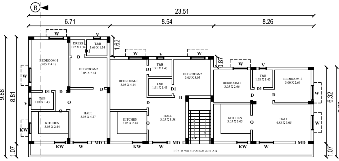
FIRST FLOOR RCC PLAN
