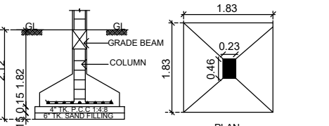
Foundation Details
