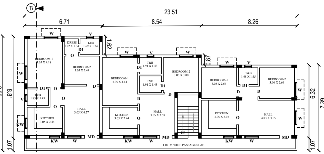
SECOND FLOOR RCC PLAN
