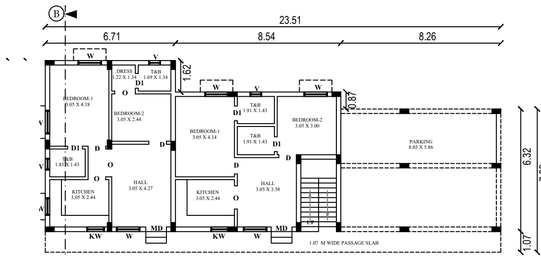
GROUND FLOOR RCC PLAN
