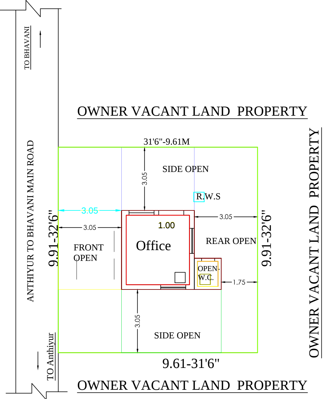
DETAILED SITE PLAN
