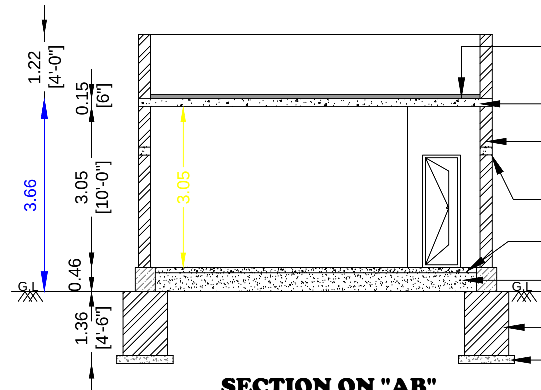
SECTION ON "AB" (SCALE 1:100)
