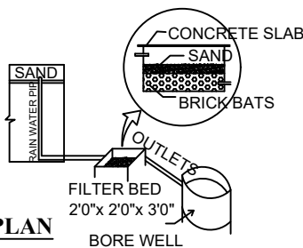
RAIN WATER HARVEST SYSTEM (NOT TO SCALE)
