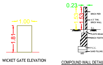
WICKET GATE ELEVATION
