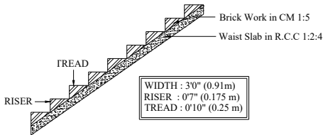
STAIRCASE DETAILS
