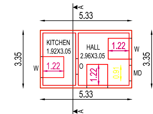
GROUND FLOOR PLAN (RESIDENTIAL BUILDING)
