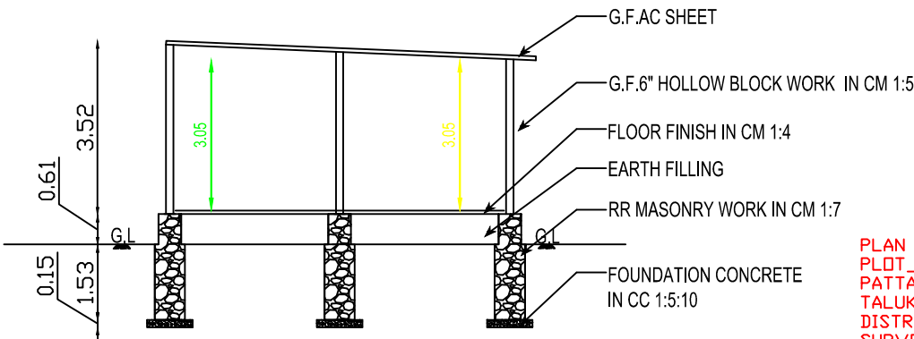
SECTION -BB
