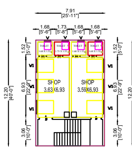
GROUND FLOOR PLAN (SOUTH)
