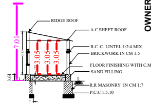
SECTION ON "MM"
