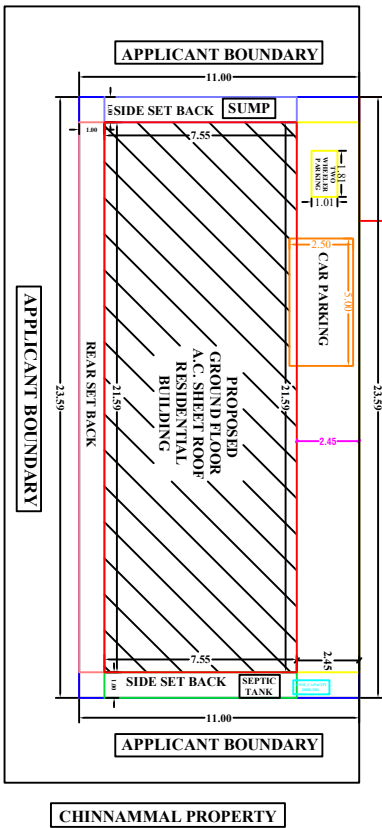
SITE PLAN
