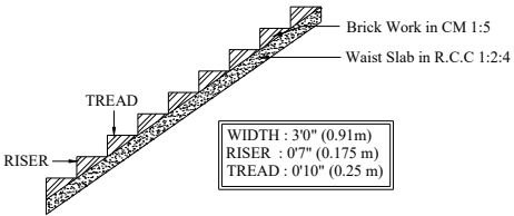
STAIRCASE DETAILS
