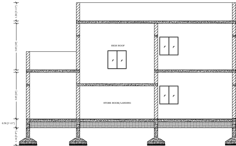
SECTION X-X
