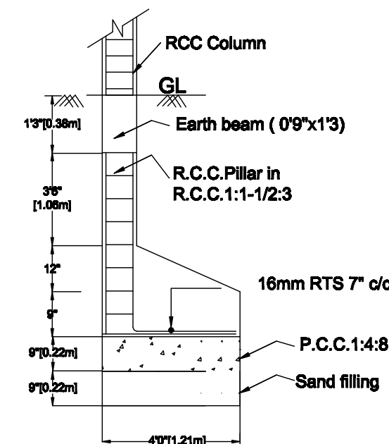
FOUNDATION DETAILS
