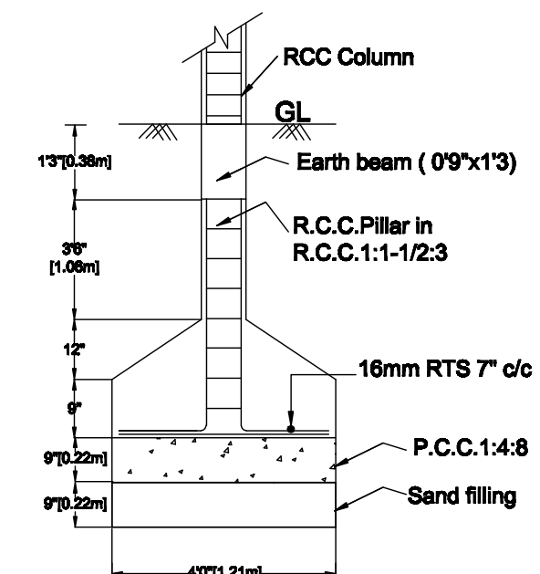
FOUNDATION DETAILS
