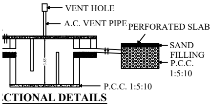
VENTILATION DETAILS
