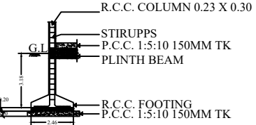
COLUMN DETAILS
