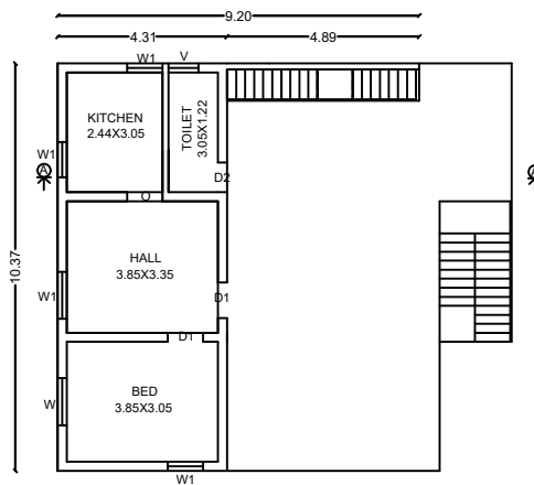
ADDITIONAL FIRST FLOOR PLAN
